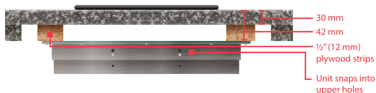
Figure 4: Incogneeto™ Unit Mounted to 1¼" (30 mm) Countertop with Two Plywood Strips
