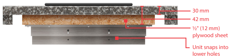
Figure 3: Incogneeto™ Unit Mounted to 1¼" (30 mm) Countertop with Plywood Sheet
